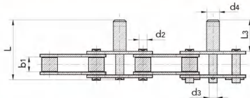
双节距加长销输送链 Double pitch conveyor chain with extended pins
