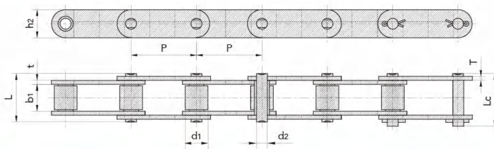
木材输送链及附件 Lumber conveyor chain & attachments
