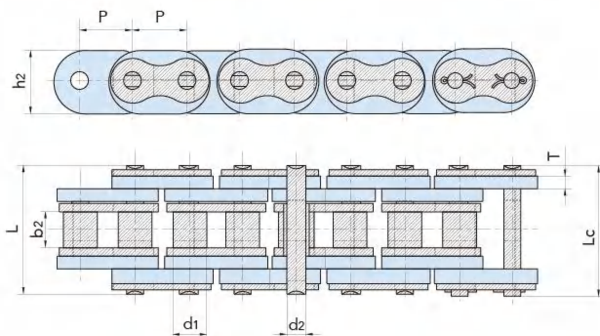
带塑料附板滚子链 Roller chain with plastic attachments
