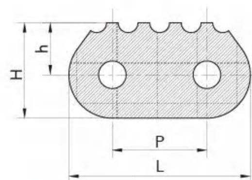
尖齿链 Sharp top chain
